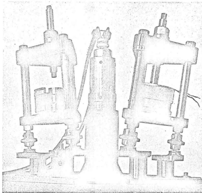
Fig. 5. Two hand presses together with the high-pressure chambers for x-raying, and with the cassettes fixed on the bench of the URS-70 x-ray apparatus.
